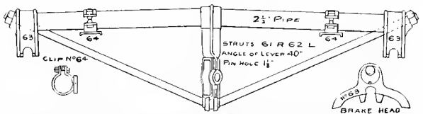
Figs. 1553-1555. Standard Rigid Head Beam for Passenger Cars and Locomotive Tenders.
